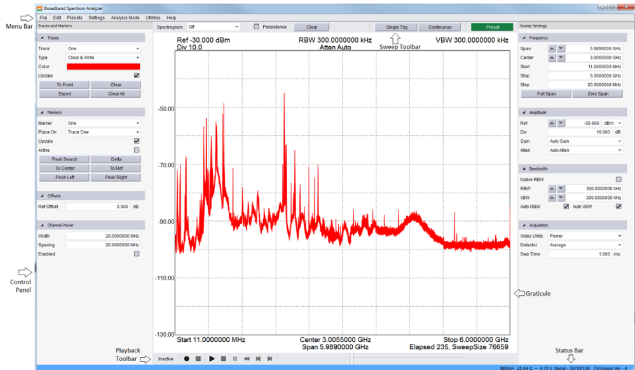
Figure 1 : The BB60 Graphical User Interface
